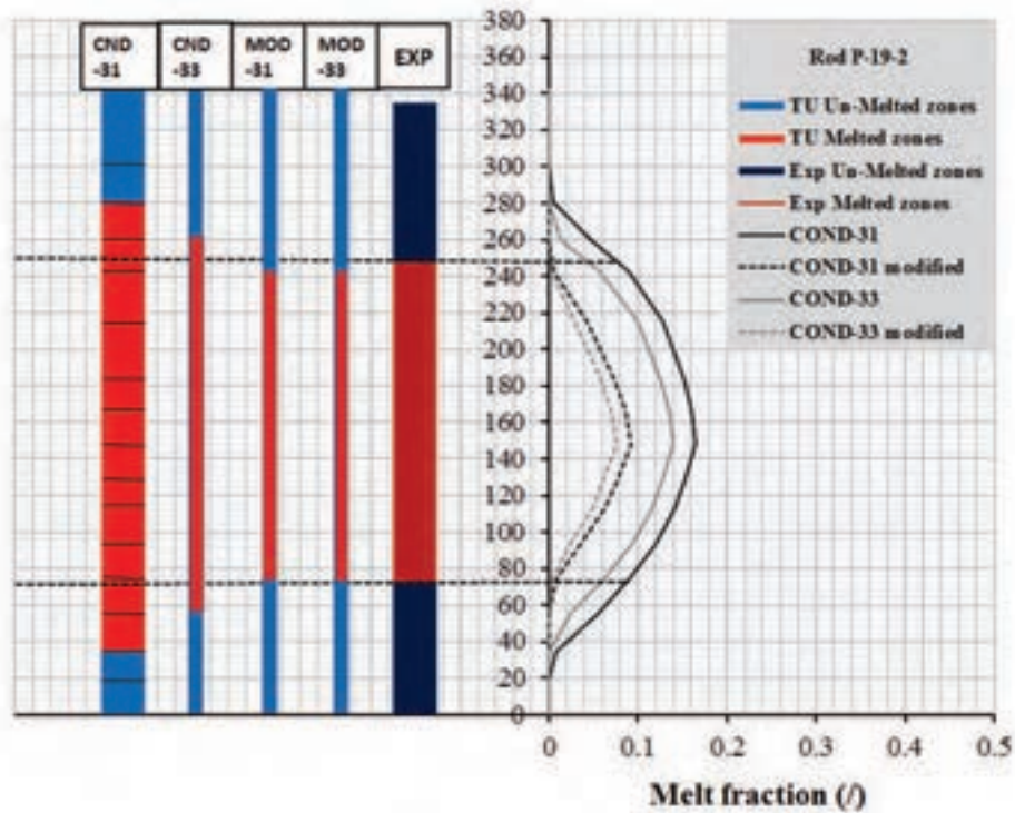
Figure 7-2 Rod P-19-2, Comparison between the melting heights and fraction according to the original and modified correlations.
