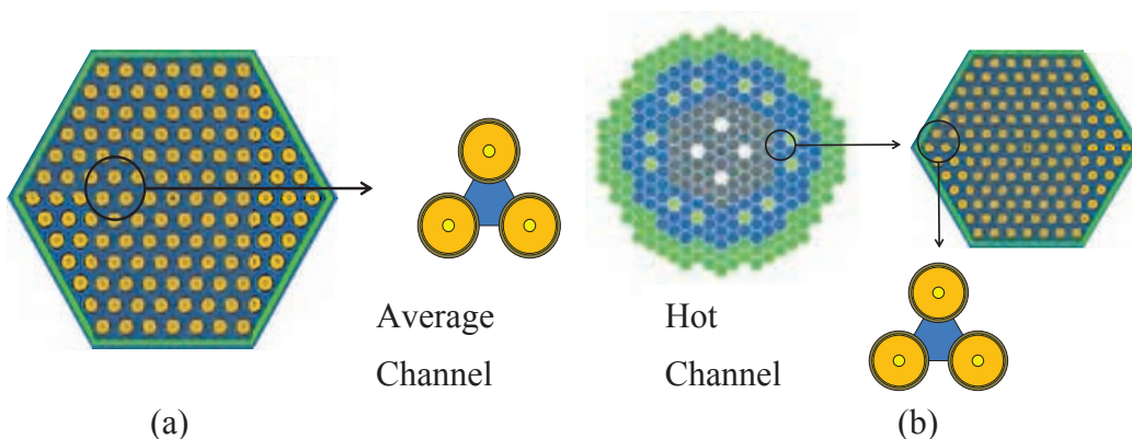
Figure 5: Graphical representation of the position of the AC (a) and the HC (b) within ALFRED core.
