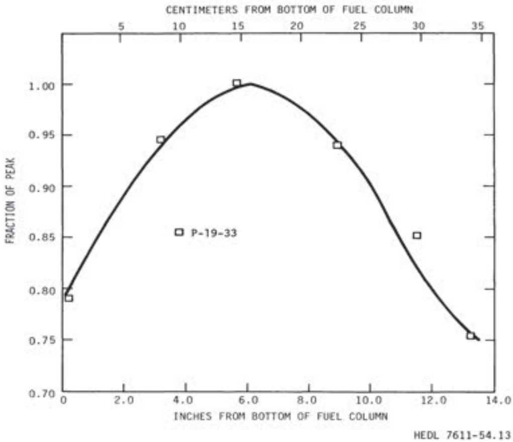
Figure 6-1 HEDL P-19, pin power axial profile. [3]
