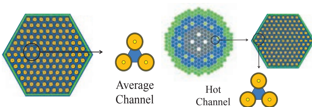
Figure 5: Graphical representation of the position of the AC (a) and the HC (b) within ALFRED core.
