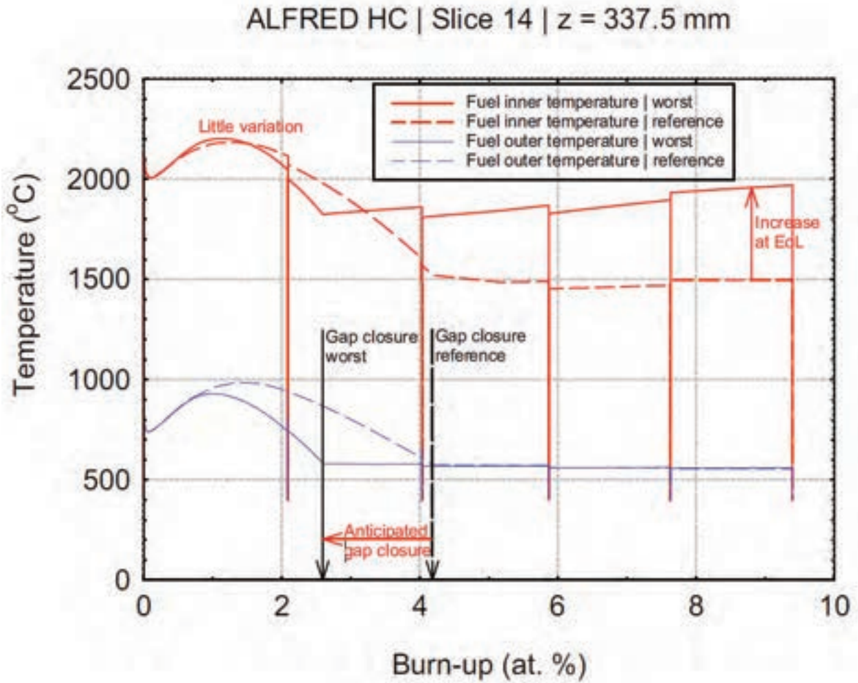
Figure 13: Comparison between ALFRED HC reference case and worst case: fuel temperature evolution.
