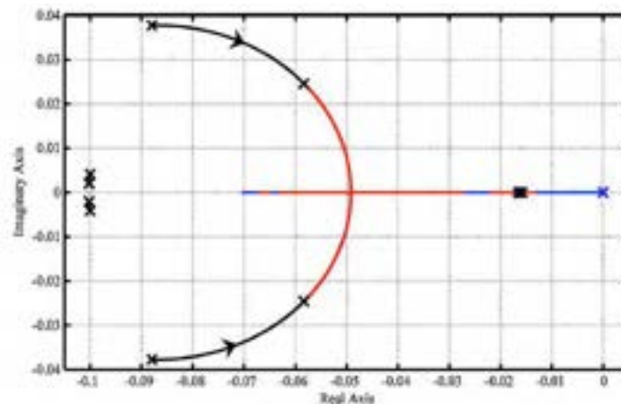
Figure 9 – root locus for the primary system as a function of power level with lead density coefficient ranging between 0 and 7 pcm/K at BoC, in ideal perfect exchange conditions.
