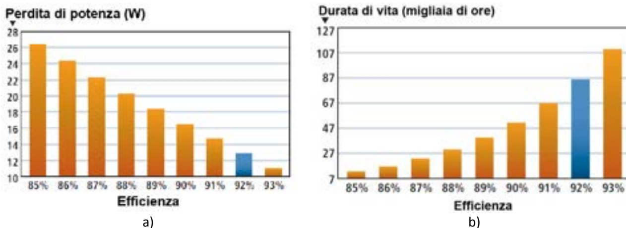
Figura 3.2. Driver LED.
