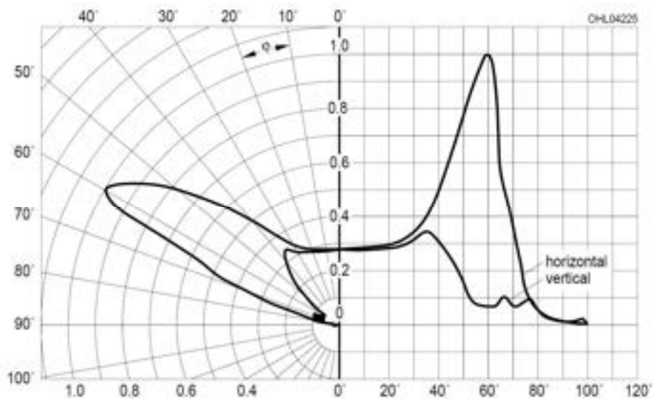
Figura 5.13. Luxeon Oval Plus, curve fotometriche.
