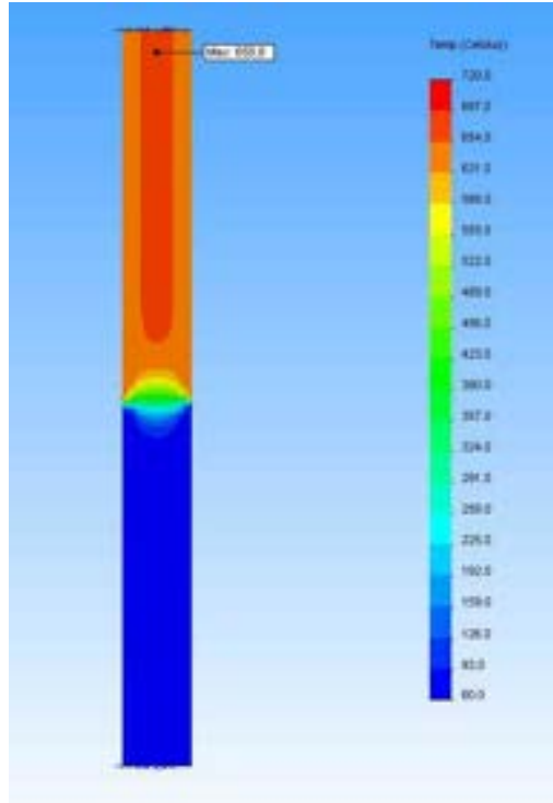
Temperature in cold part of normal rod, 20% power
